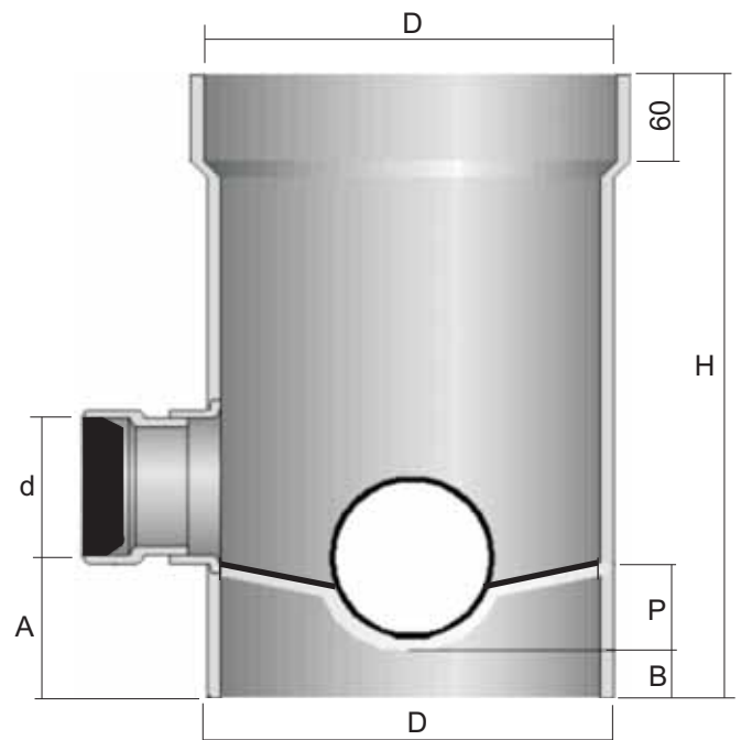
Section perpendicular to flow direction
